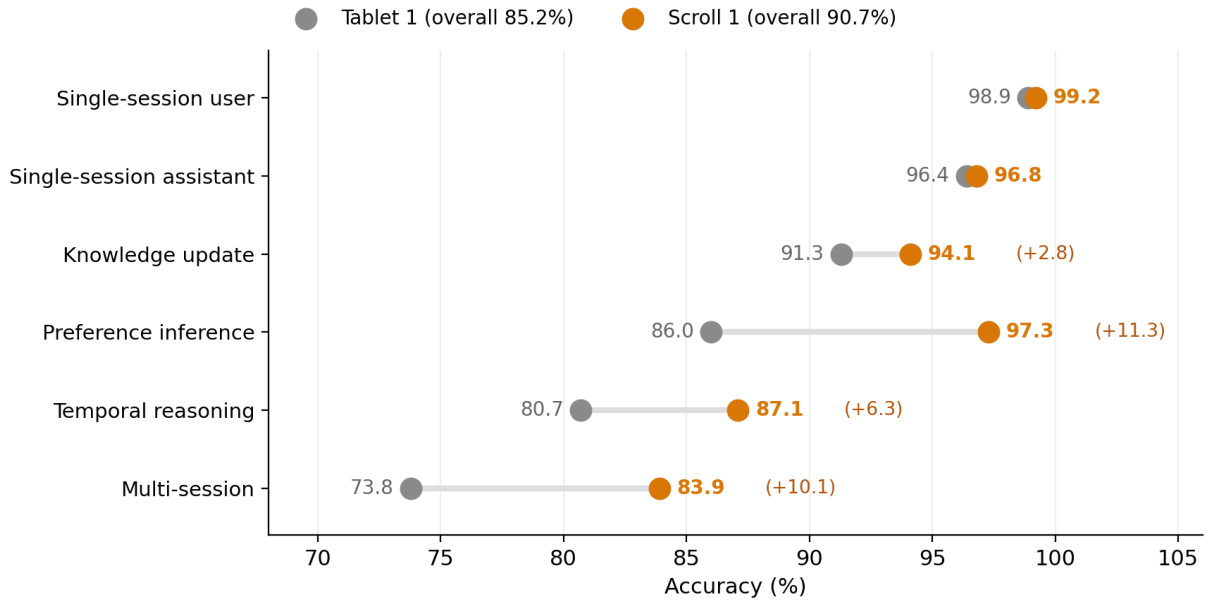
Figure 1. Per-category accuracy, five-run means (LongMemEval-S)
